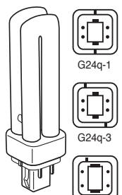
G24q base Quad Tube
